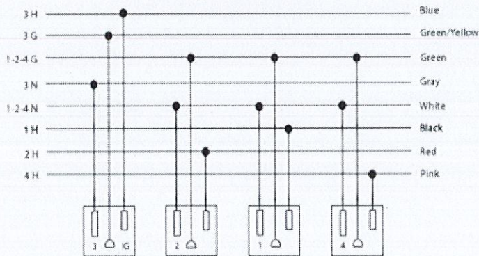
Electri-Pak 8 Wire, 4 Circuit Wiring Schematic
